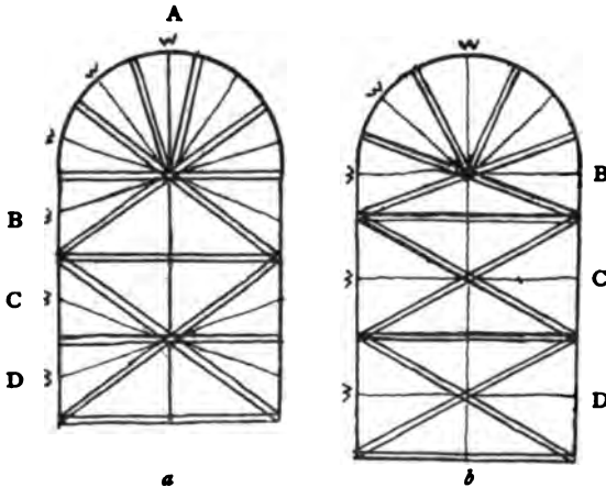
FIG. 65. Diagrams of vaults.
